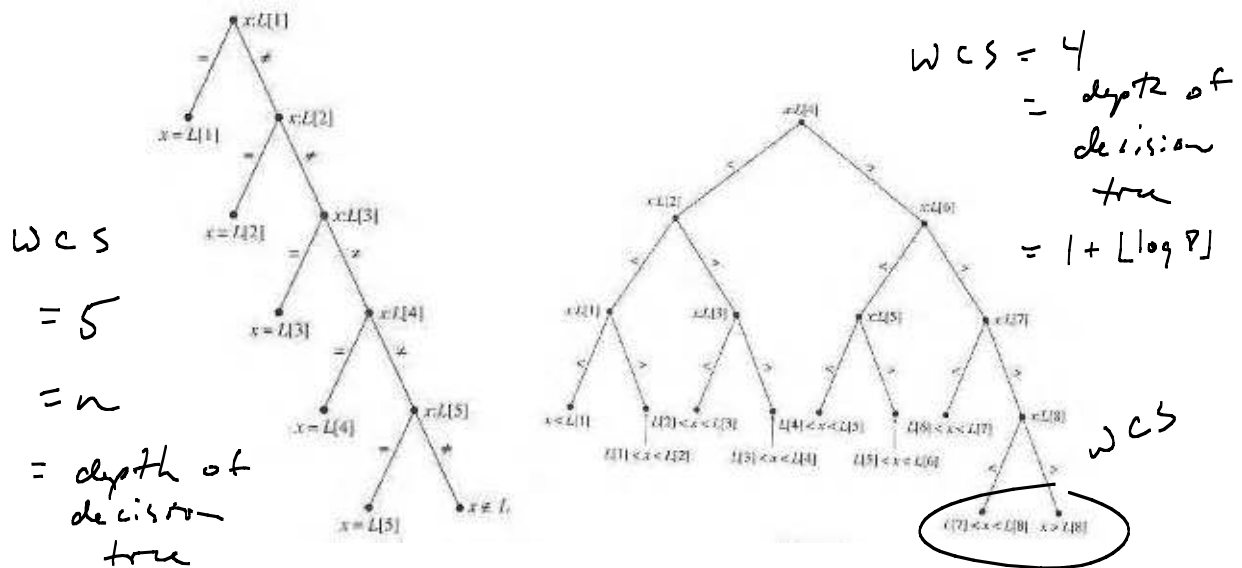
Figure 2: Figure 5.52, p. 388/453: Sequential Search on 5 elements (binary tree); Figure 5.53, p. 389/454: Binary Search on a sorted list (ternary tree, although it appears binary since those leaves corresponding to equality have been suppressed). Notice how clumsy this binary tree looks, since a power of two was used (8 elements), rather than one less than a power of two ( 7=2^3 - 1 ).
