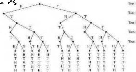
Figure 1: Figure 5.51, p. 387/452: Results of tossing a coin 5 times, no two heads in a row (binary decision tree)
