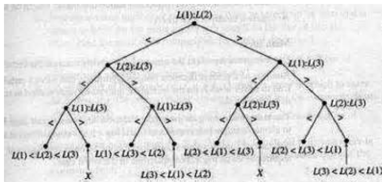
Figure 4: Figure 5.56, p. 393/457: Sorting a list (binary tree, provided distinct list elements)
