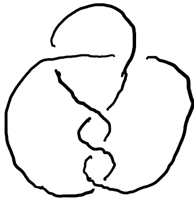
5-crossing twist knot
